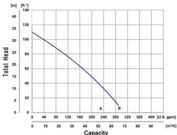
Performance of Engine Driven Self-Priming Trash Pump
