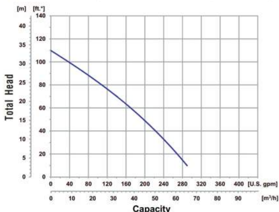
Performance of Engine Driven Self-Priming Trash Pumps
